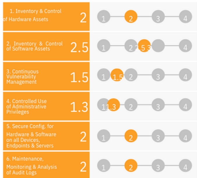
CISv7 Basic
